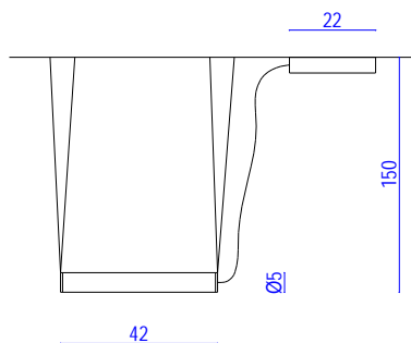
NEVADA 40 230V AC LED 12W 24V zintegrowane CE \nabla IP20 \oplus
